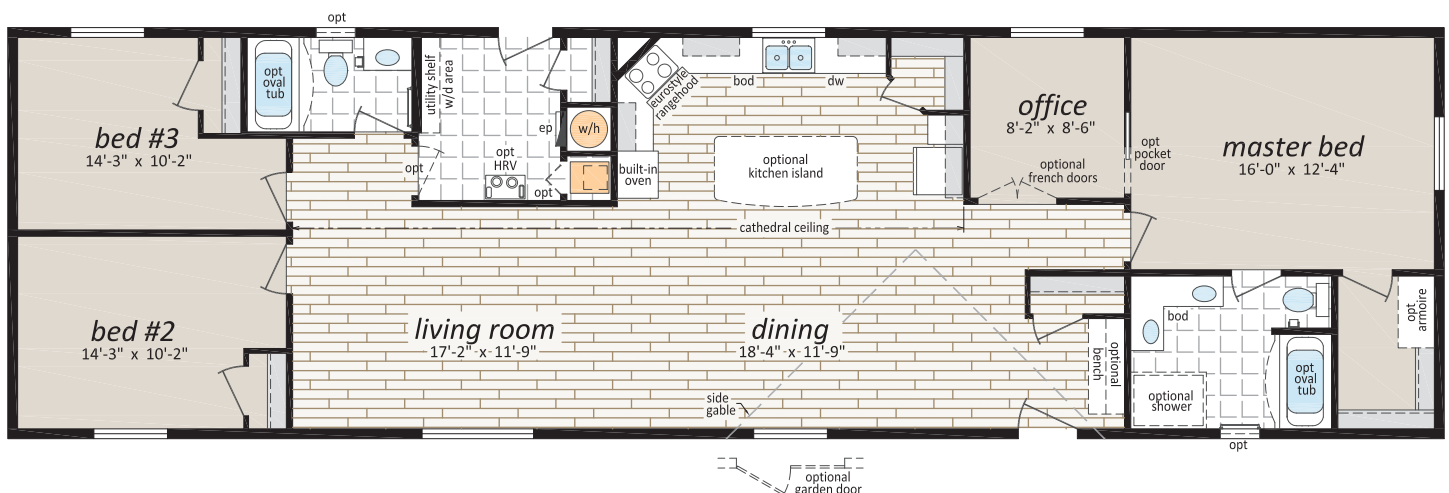
MT-227603 22' x 76' - 1,672 SQ.FT. 3 BEDS, 2 BATHS, OFFICE
